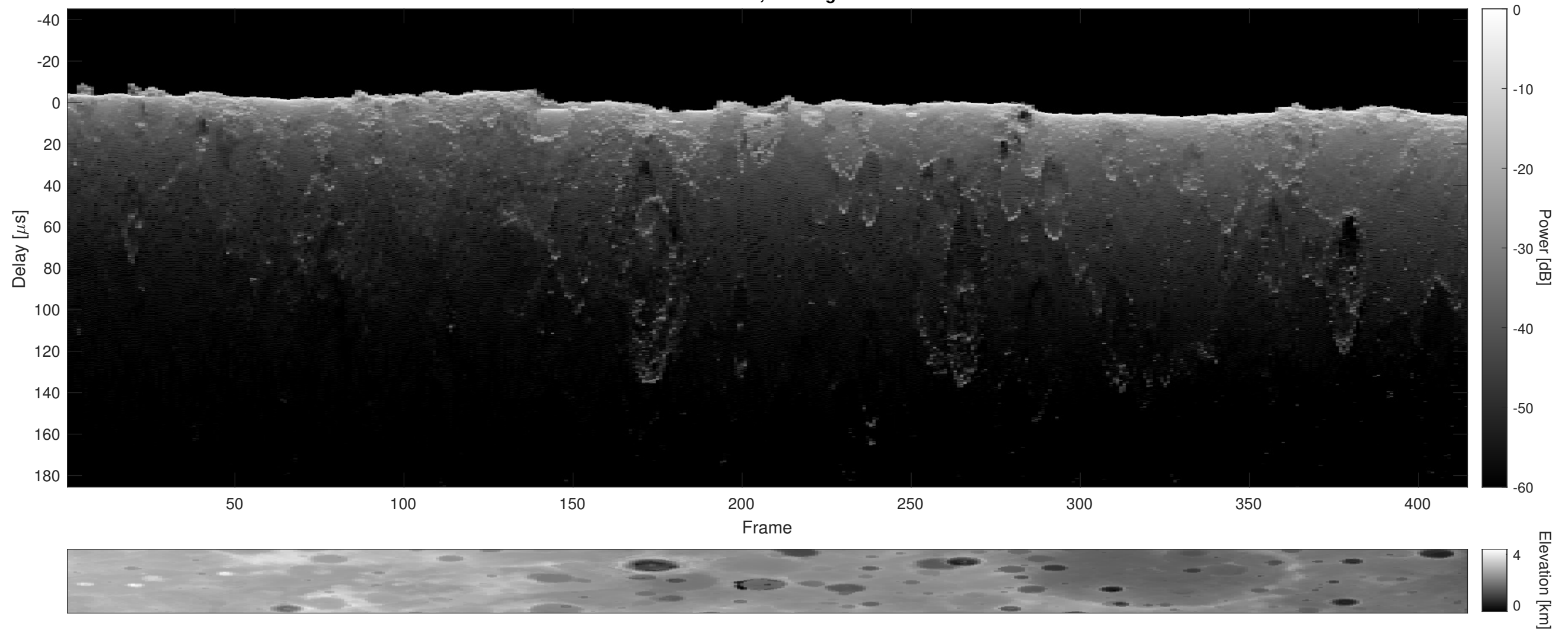
Orbit 14969, Cluttergram
