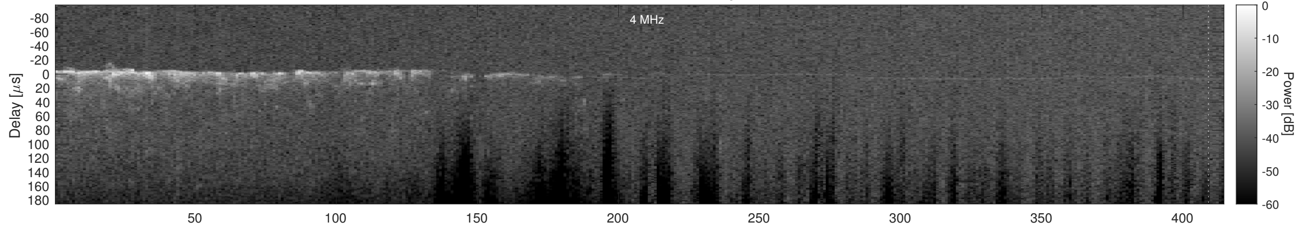
Orbit 14969, Cluttergram
