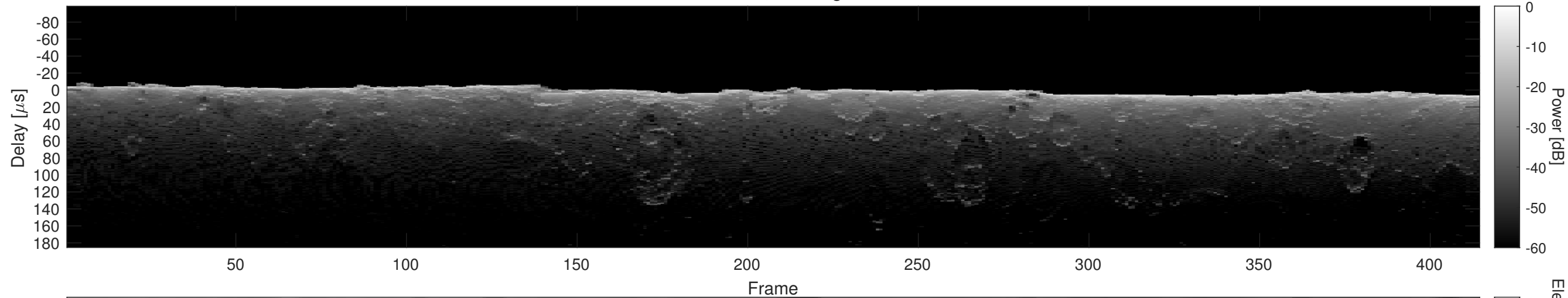
Orbit 14969, Cluttergram
