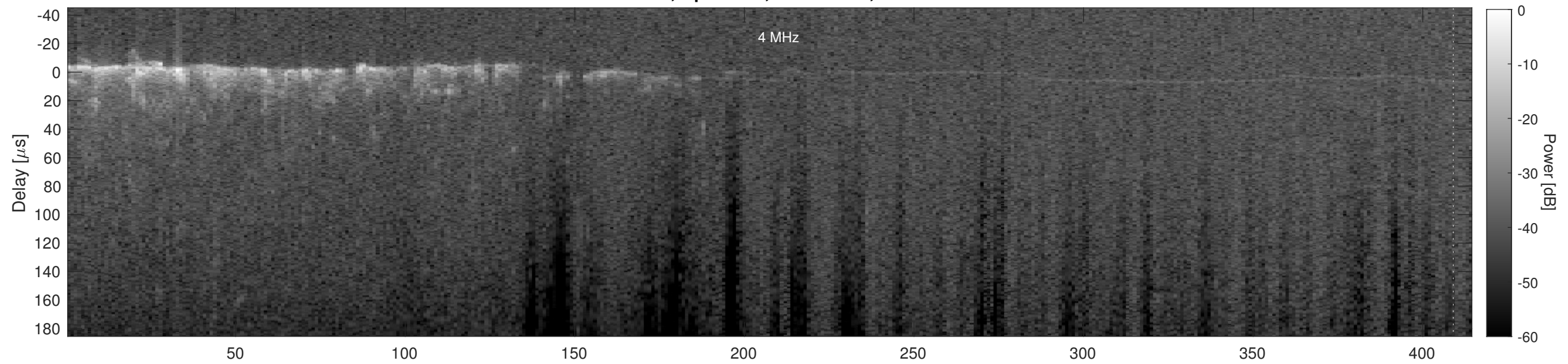
Orbit 14969, Cluttergram
