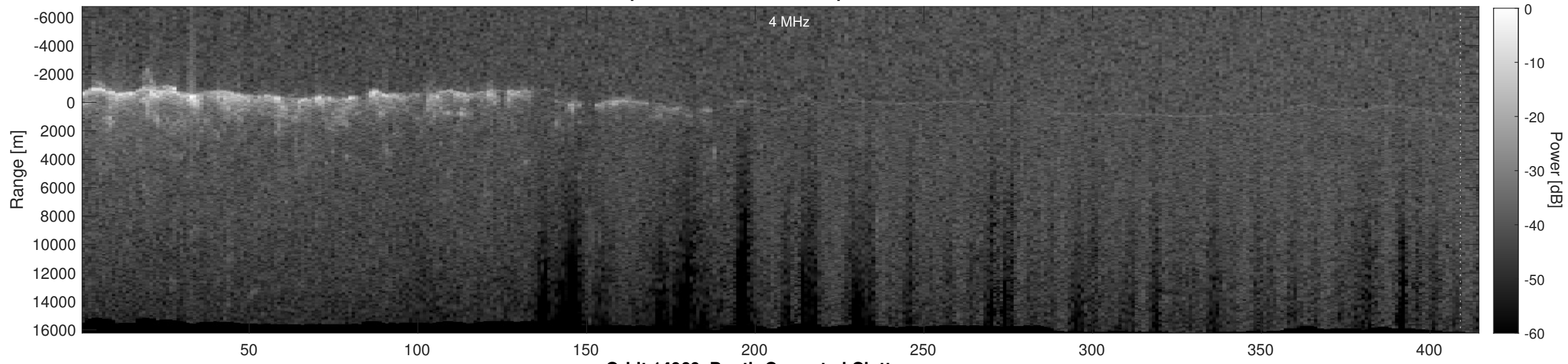
Orbit 14969, Depth-Corrected Cluttergram
