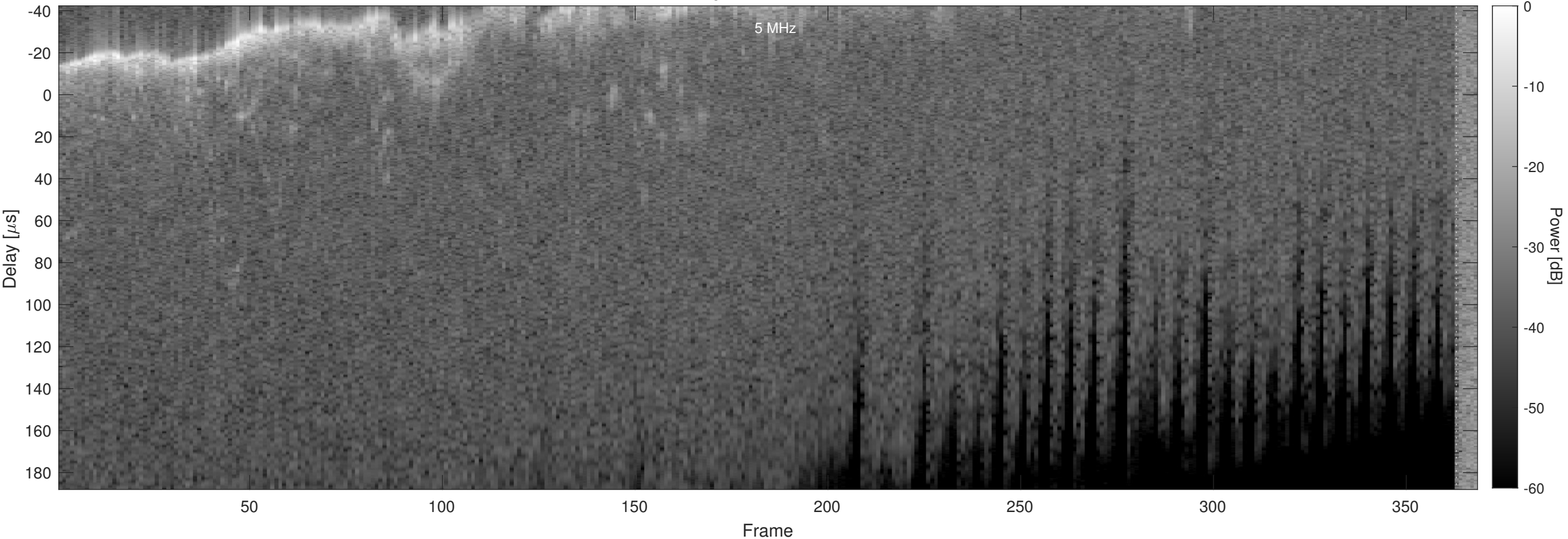
Orbit 14983, Chapman, No Window, Channel 2
