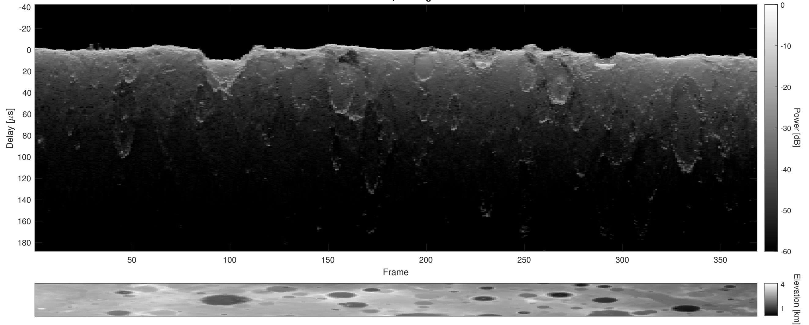
Orbit 14983, Cluttergram
