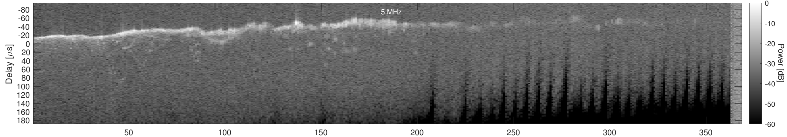
Orbit 14983, Window, Channel 1, Optimized
