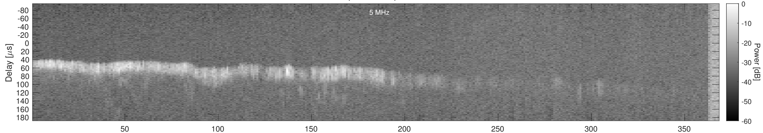
Orbit 14983, Window, Channel 1, Chapman
