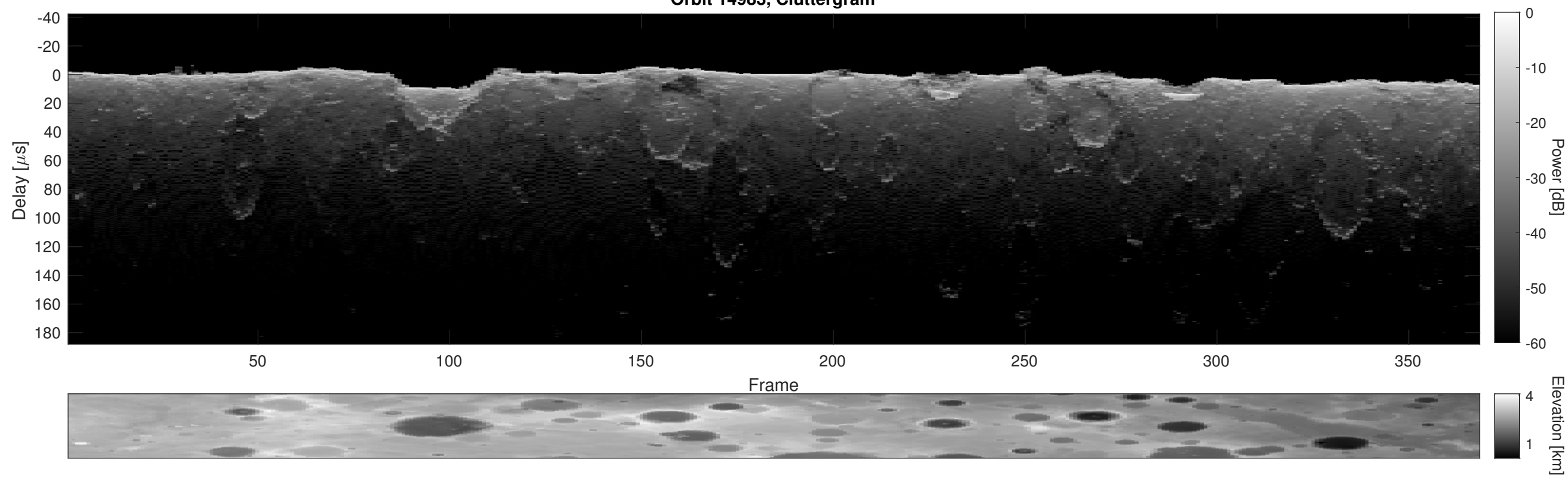
Orbit 14983, Cluttergram
