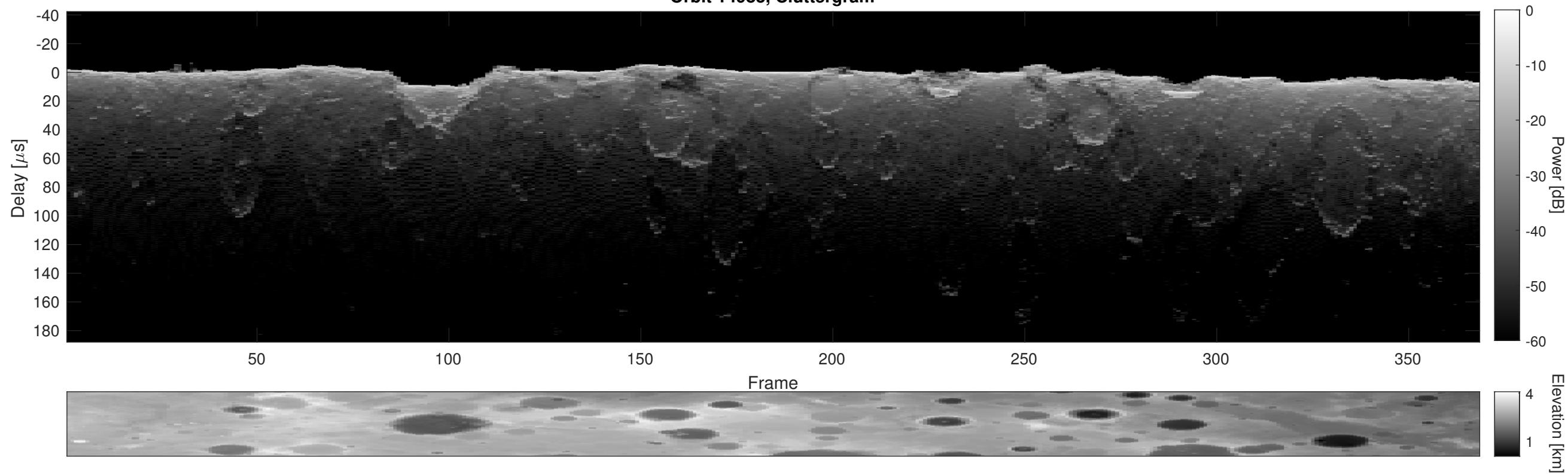
Orbit 14983, Cluttergram
