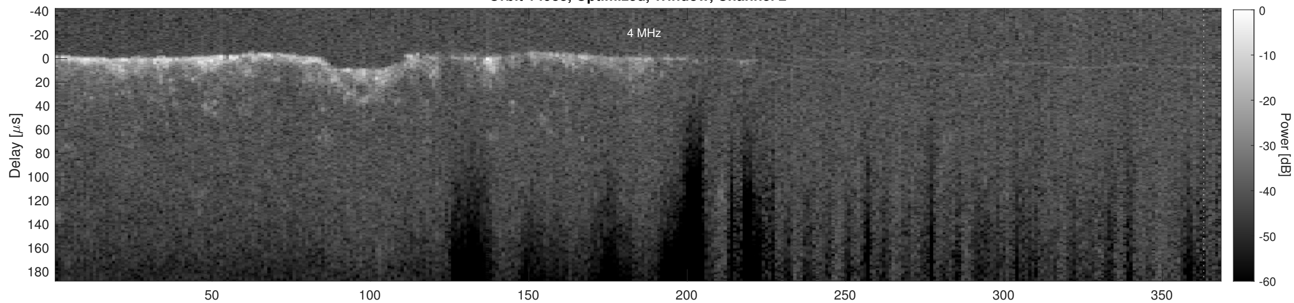
Orbit 14983, Cluttergram
