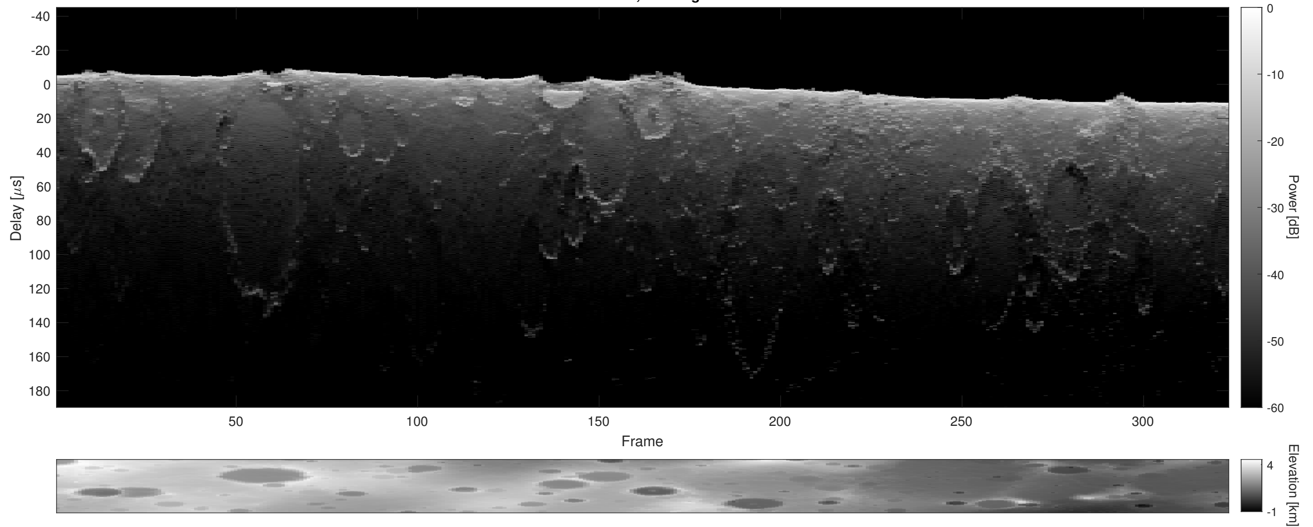
Orbit 14985, Cluttergram
