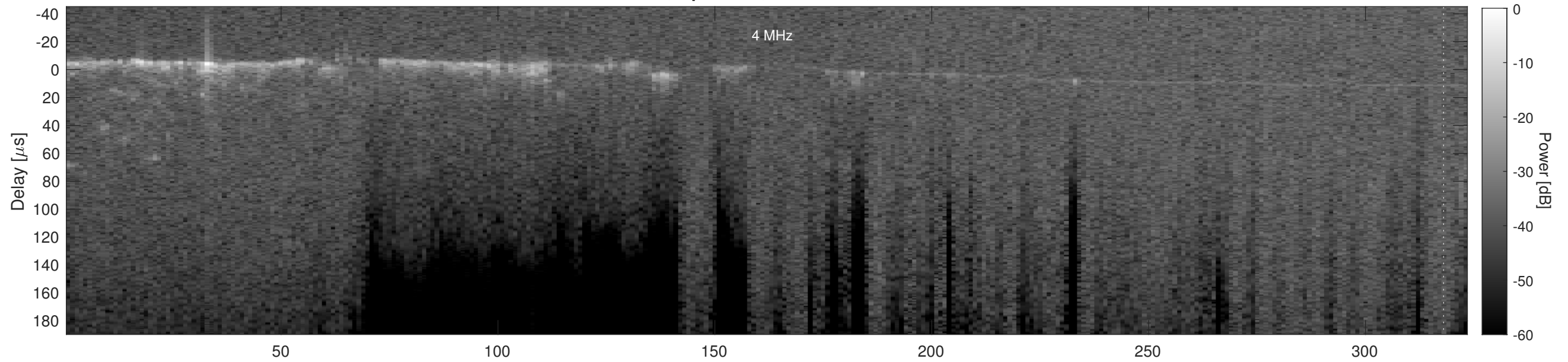
Orbit 14985, Cluttergram
