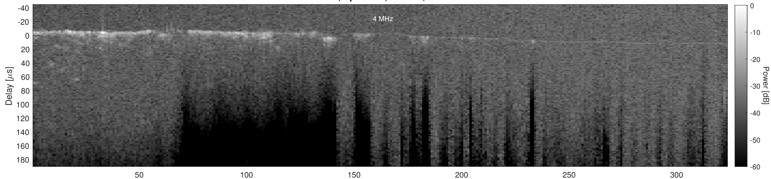
Orbit 14985, Cluttergram
