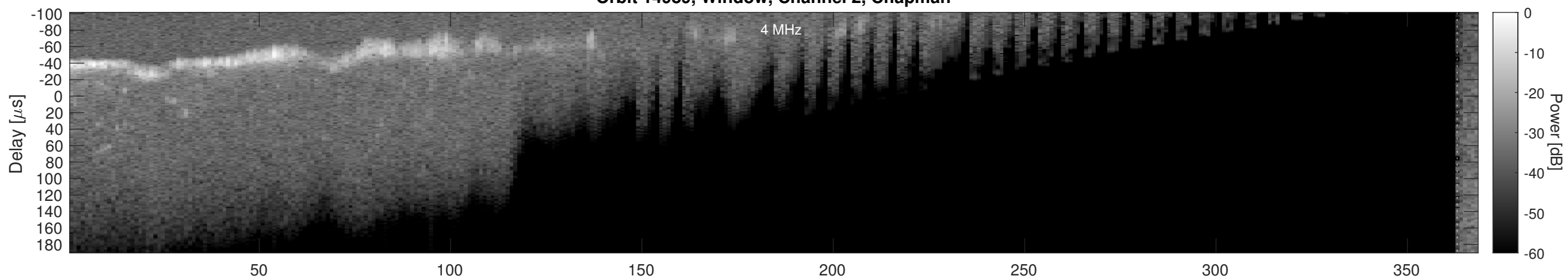
Orbit 14989, Window, Channel 2, Optimized
