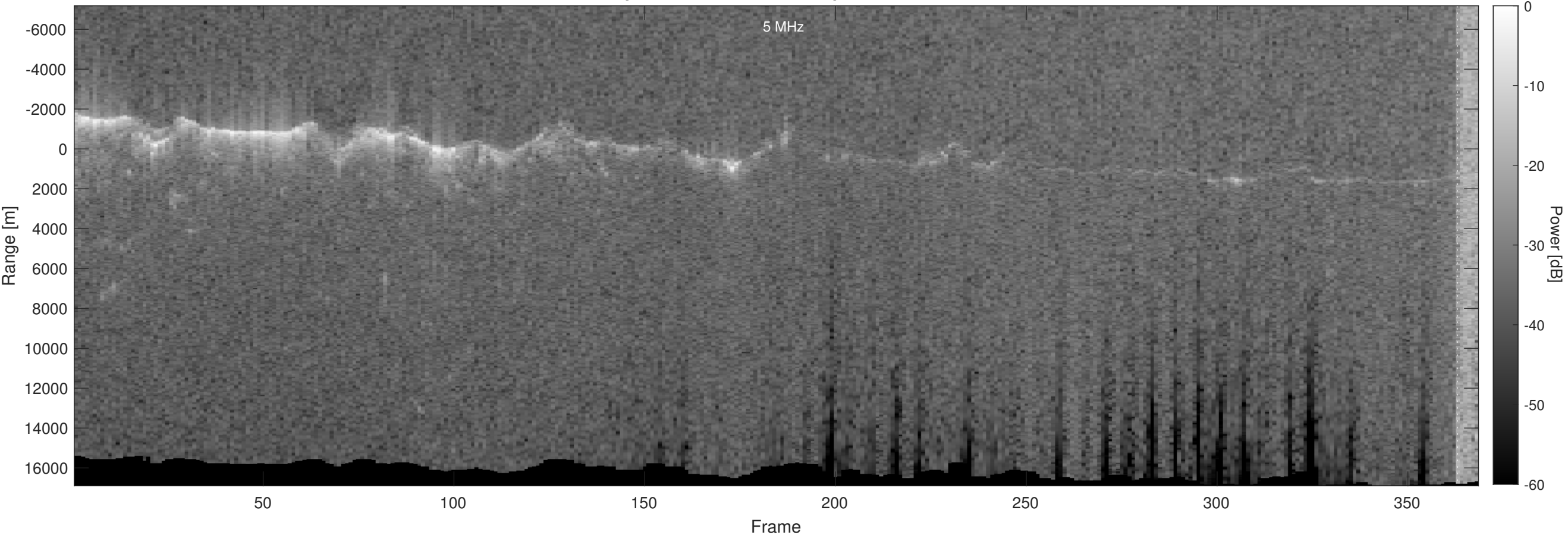
Orbit 14989, Optimized, No Window, Depth-Corrected, Channel 2
