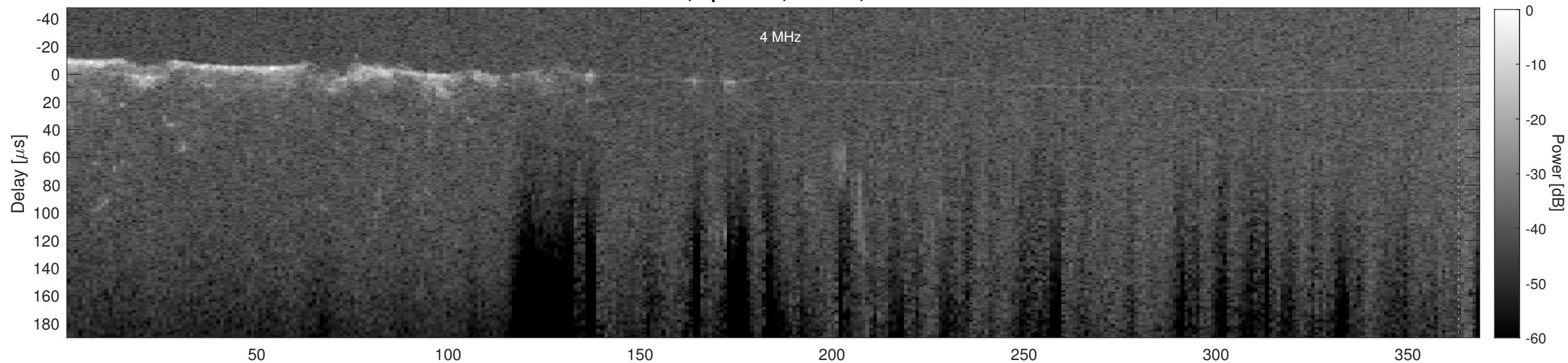
Orbit 14989, Cluttergram
