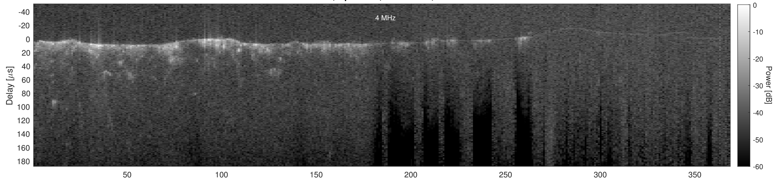
Orbit 14991, Cluttergram
