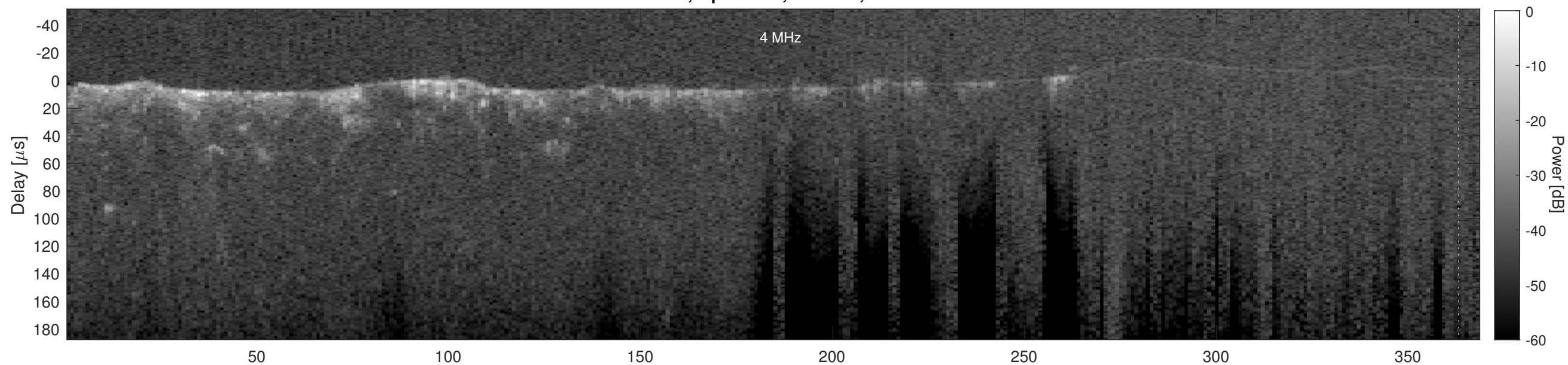
Orbit 14991, Cluttergram
