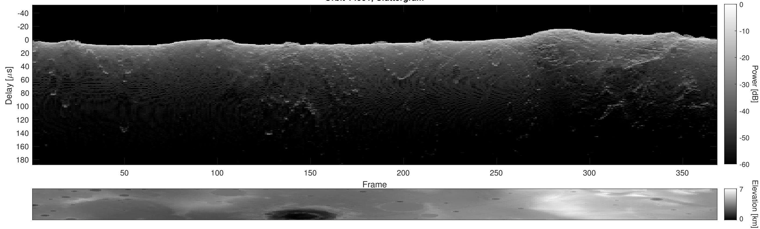
Orbit 14991, Cluttergram
