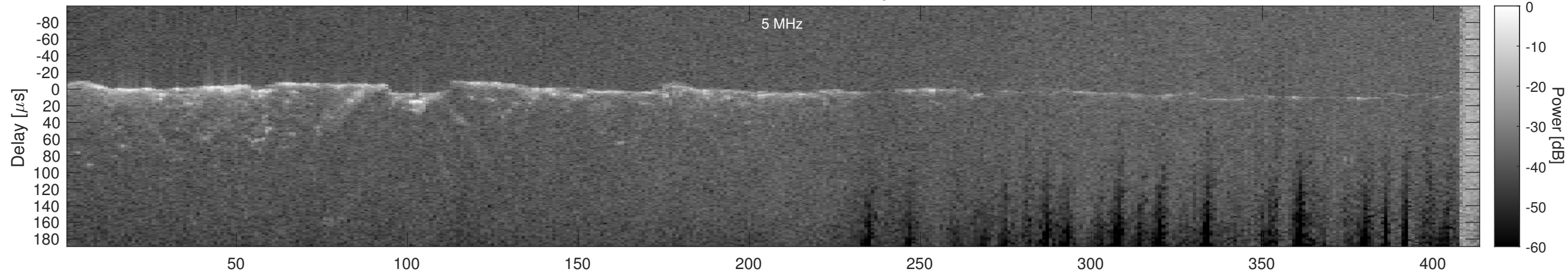
Orbit 14996, Cluttergram
