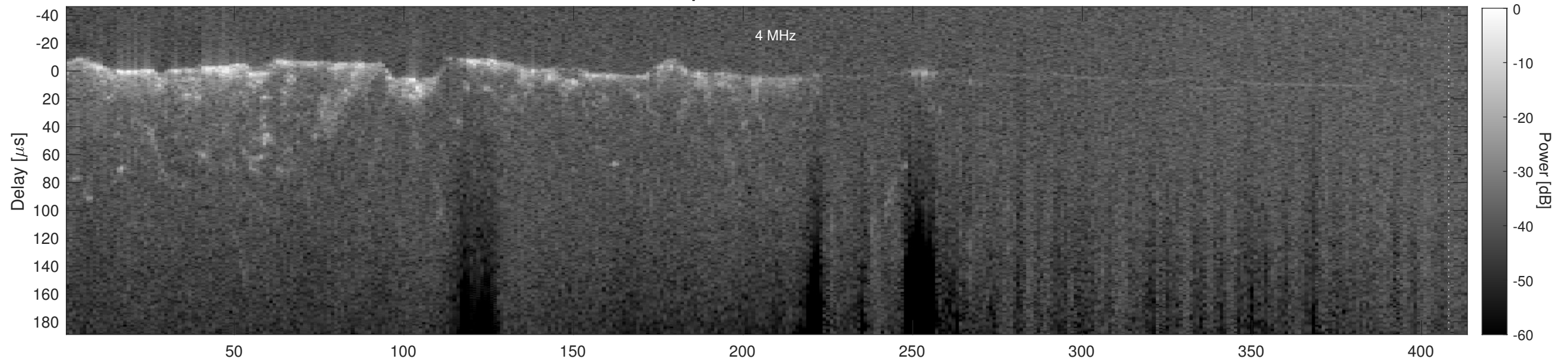
Orbit 14996, Cluttergram
