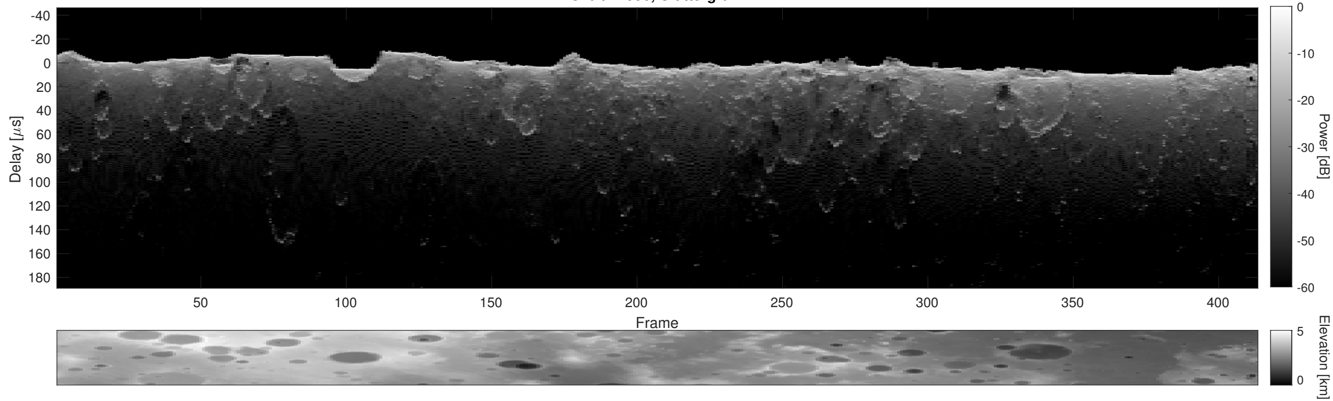
Orbit 14996, Cluttergram
