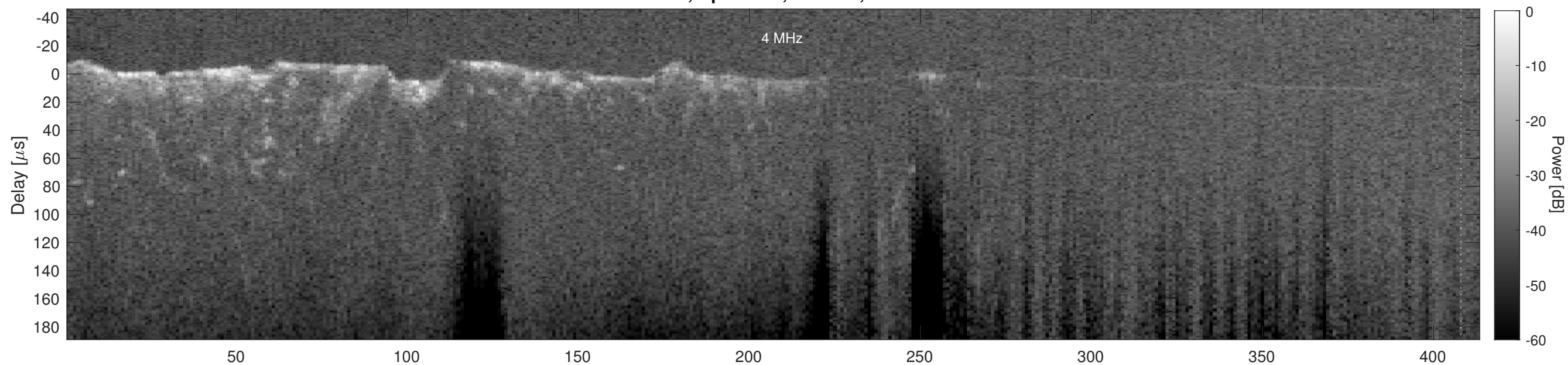
Orbit 14996, Cluttergram
