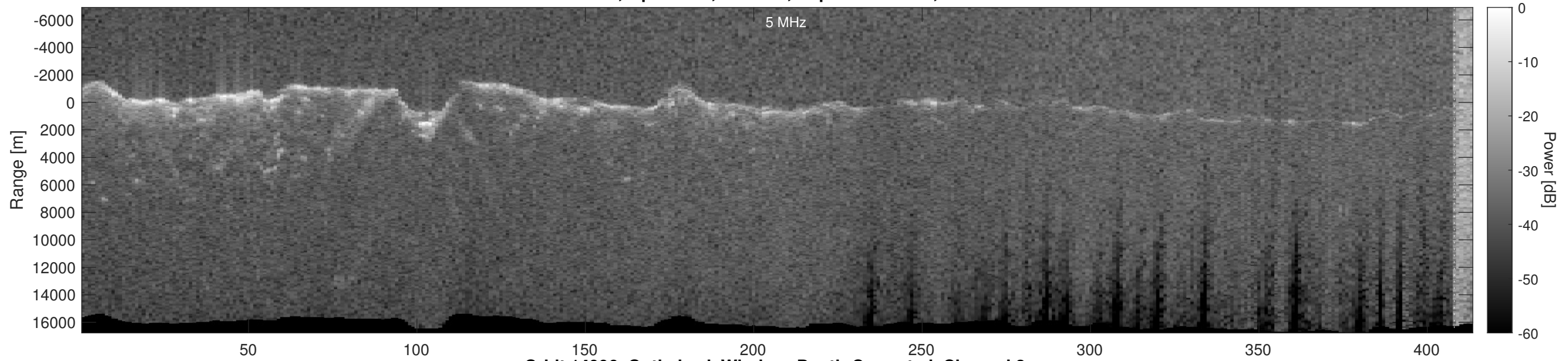
Orbit 14996, Optimized, Window, Depth-Corrected, Channel 2
