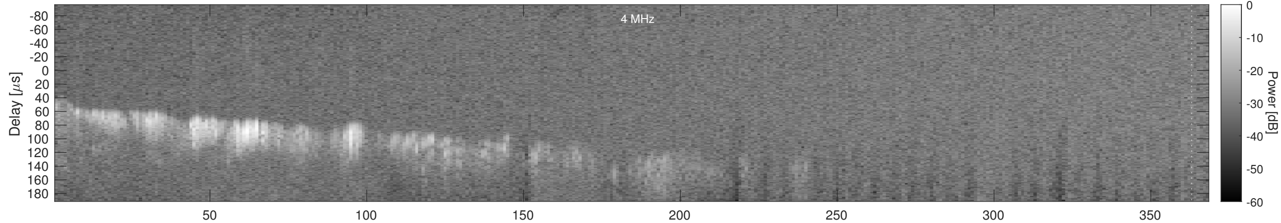
Orbit 14999, Window, Channel 2, Chapman
