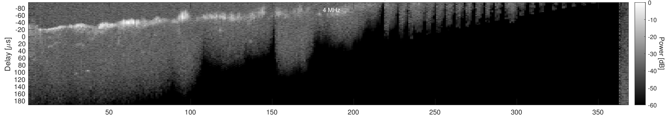
Orbit 14999, Window, Channel 2, Optimized
