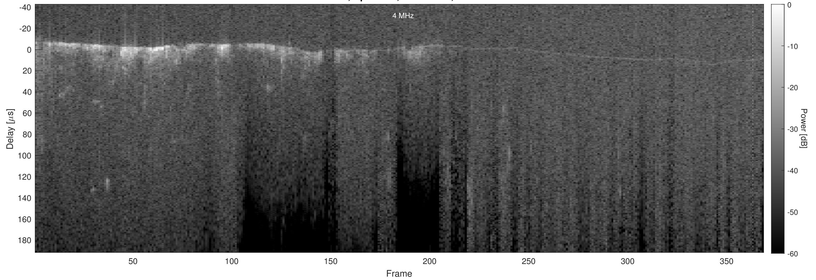
Orbit 14999, Optimized, No Window, Channel 2
