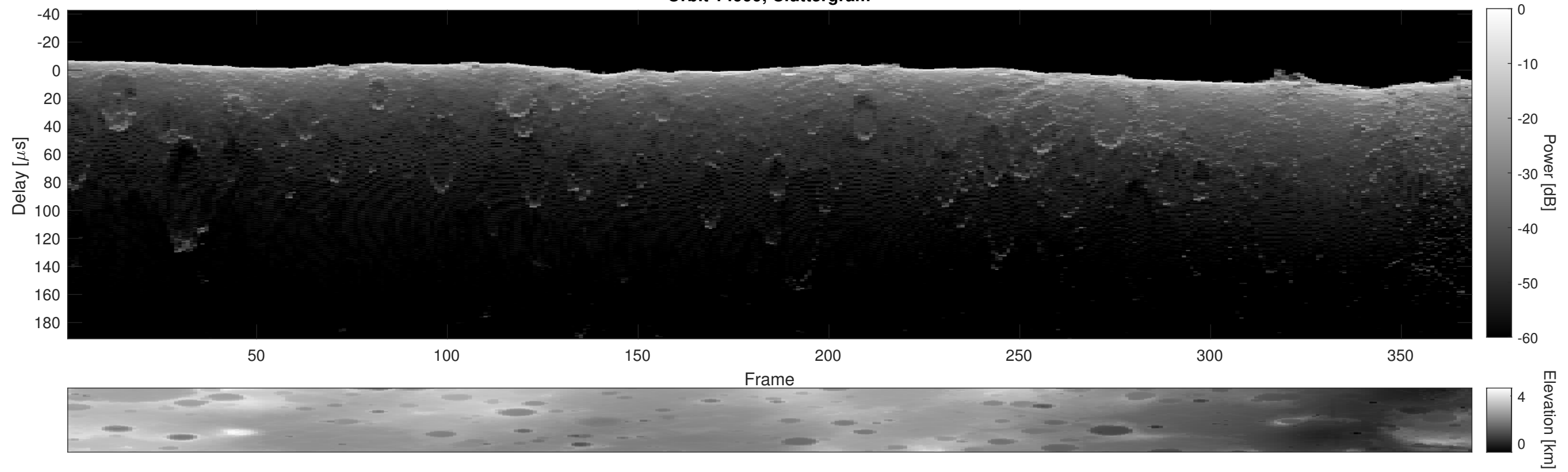
Orbit 14999, Cluttergram
