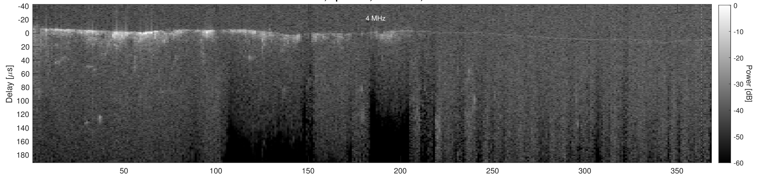
Orbit 14999, Cluttergram
