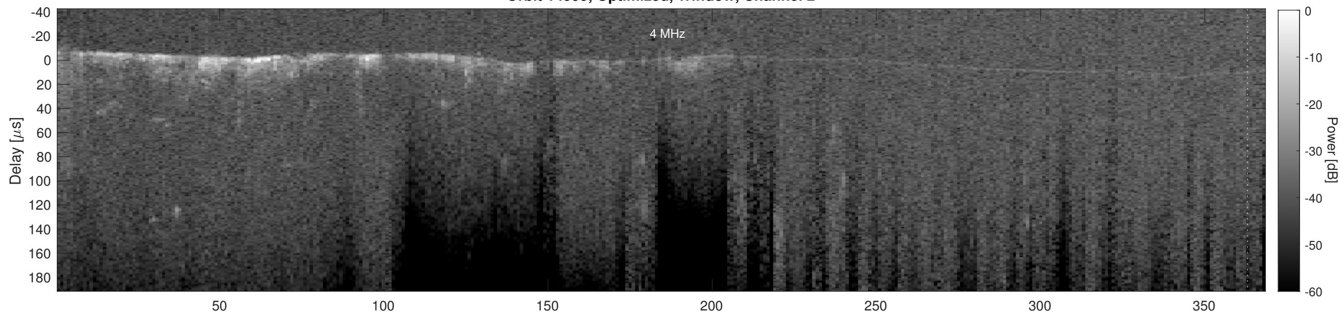
Orbit 14999, Cluttergram
