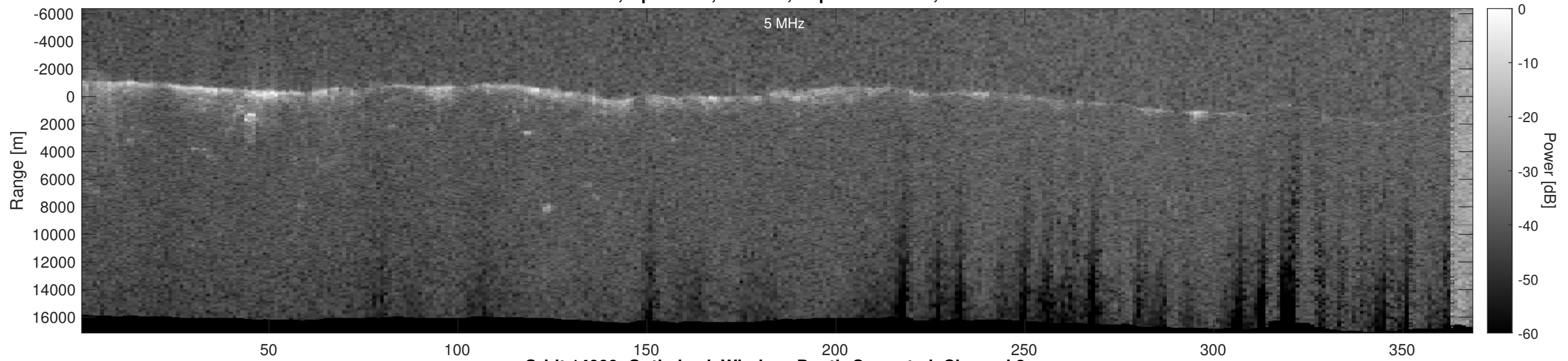
Orbit 14999, Optimized, Window, Depth-Corrected, Channel 2
