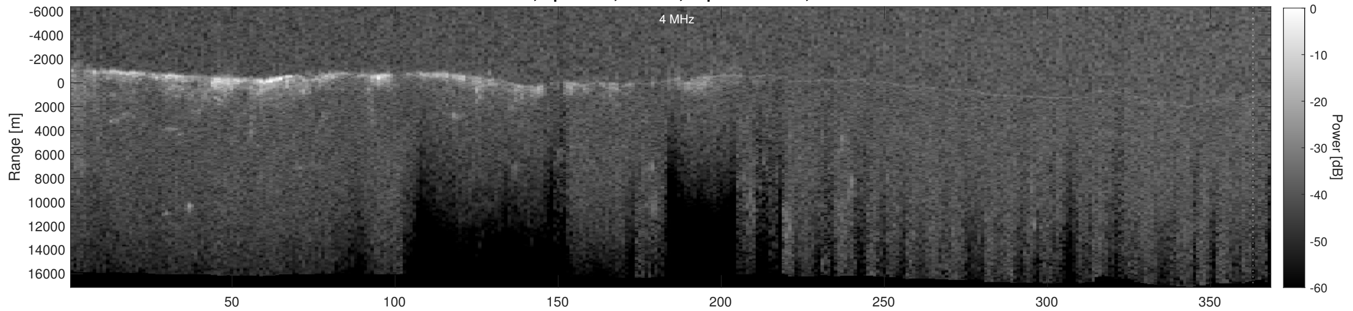
Orbit 14999, Depth-Corrected Cluttergram
