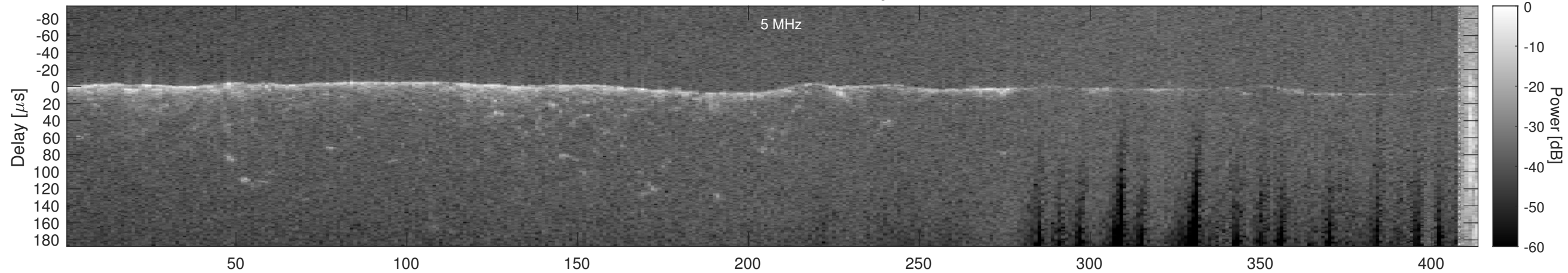
Orbit 15003, Cluttergram
