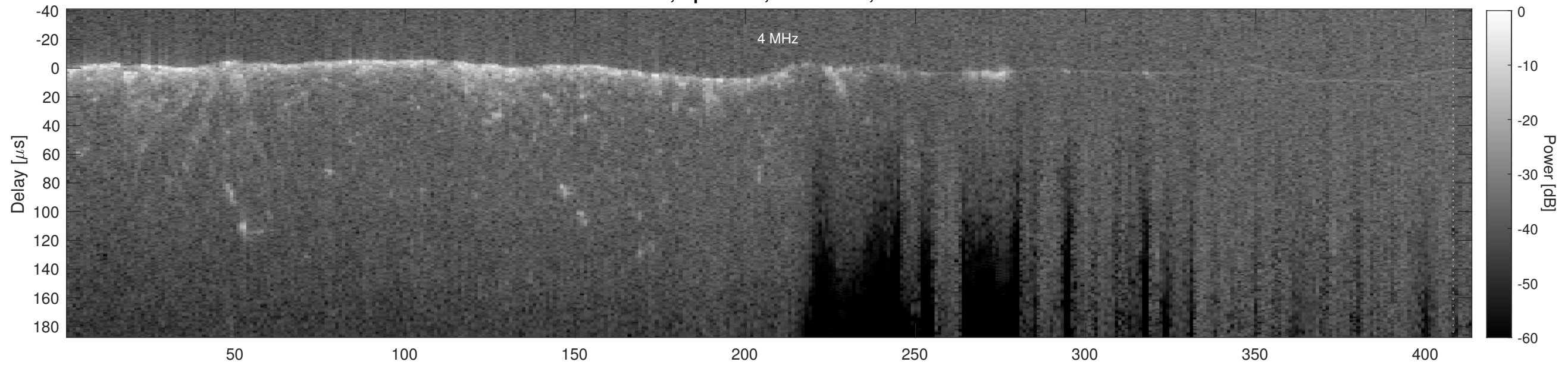
Orbit 15003, Cluttergram
