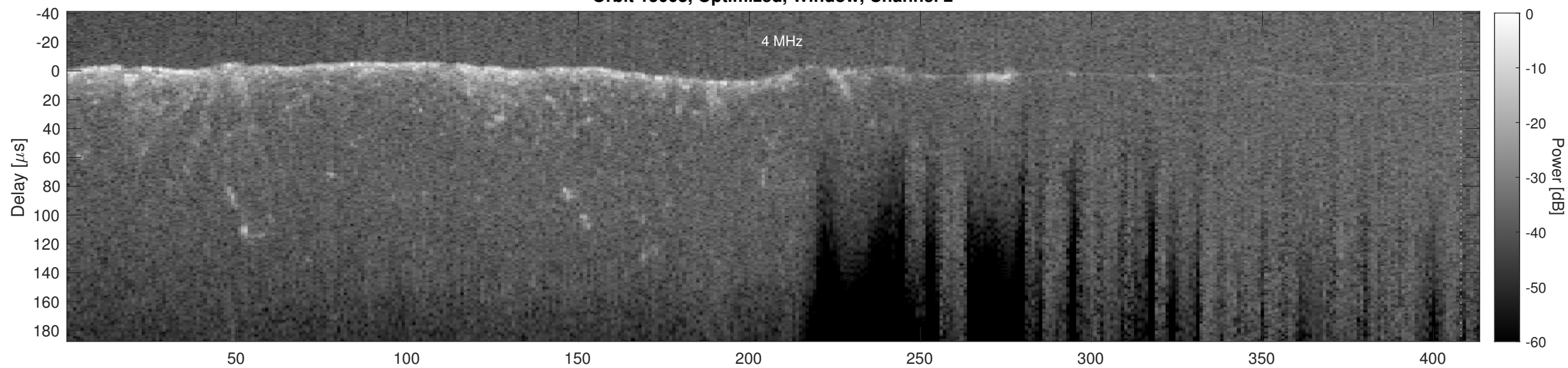
Orbit 15003, Cluttergram
