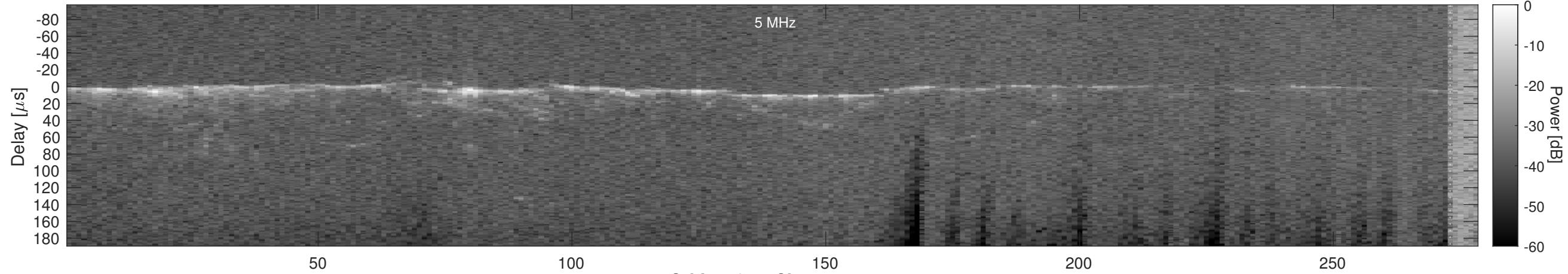
Orbit 15011, Cluttergram
