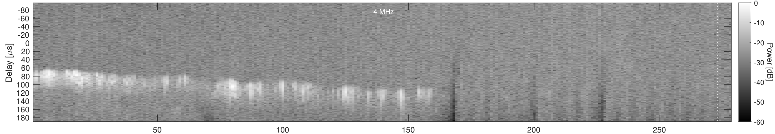
Orbit 15011, Window, Channel 2, Chapman
