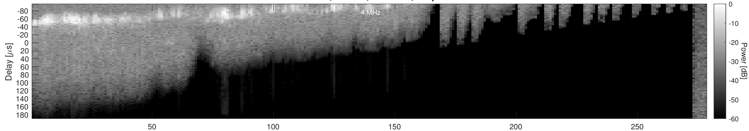
Orbit 15011, Window, Channel 2, Optimized
