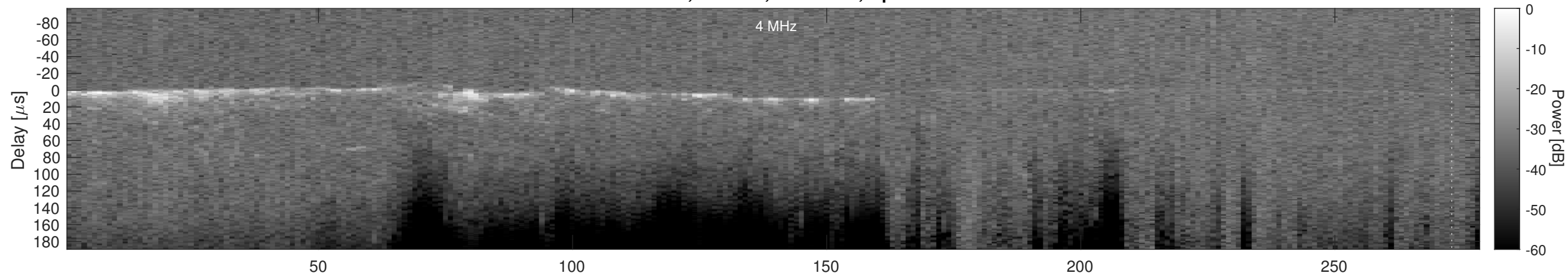
Orbit 15011, Cluttergram
