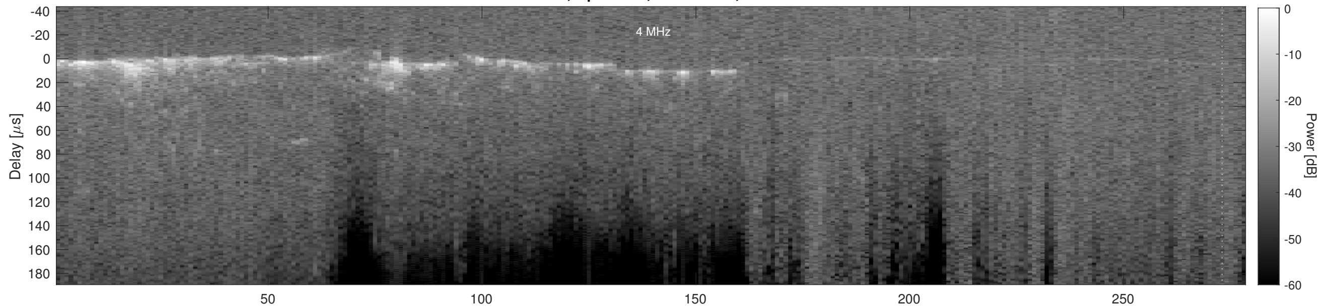
Orbit 15011, Cluttergram
