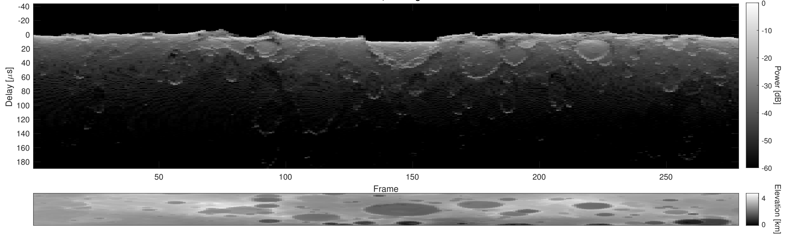
Orbit 15011, Cluttergram
