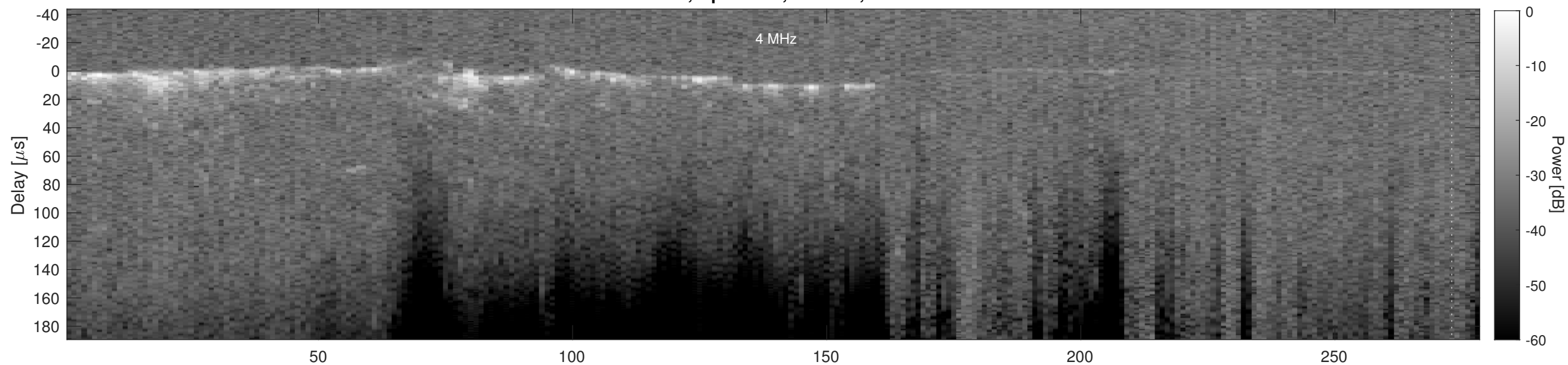
Orbit 15011, Cluttergram
