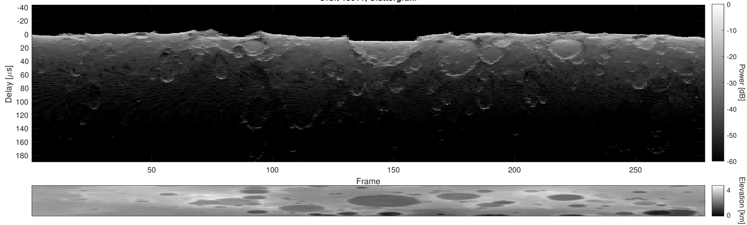
Orbit 15011, Cluttergram
