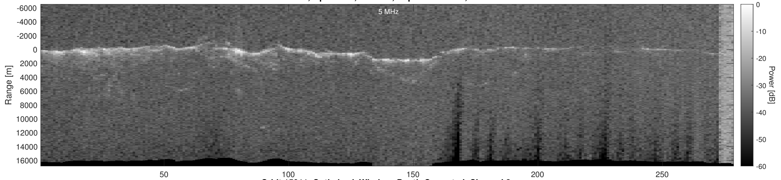
Orbit 15011, Optimized, Window, Depth-Corrected, Channel 2
