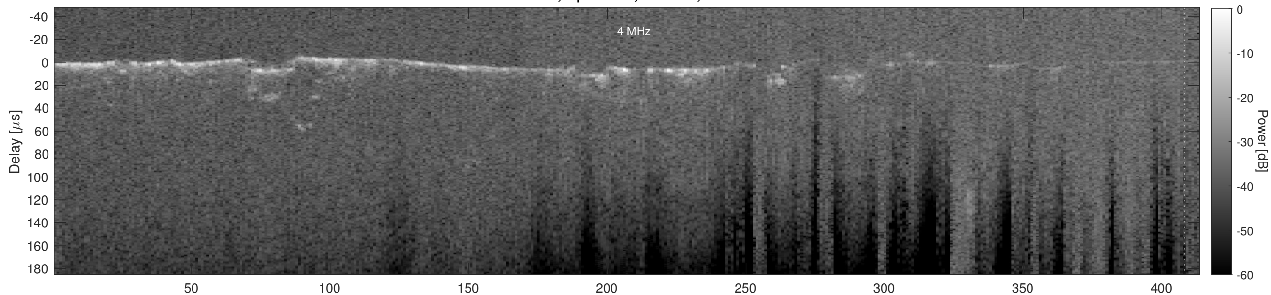
Orbit 15030, Cluttergram
