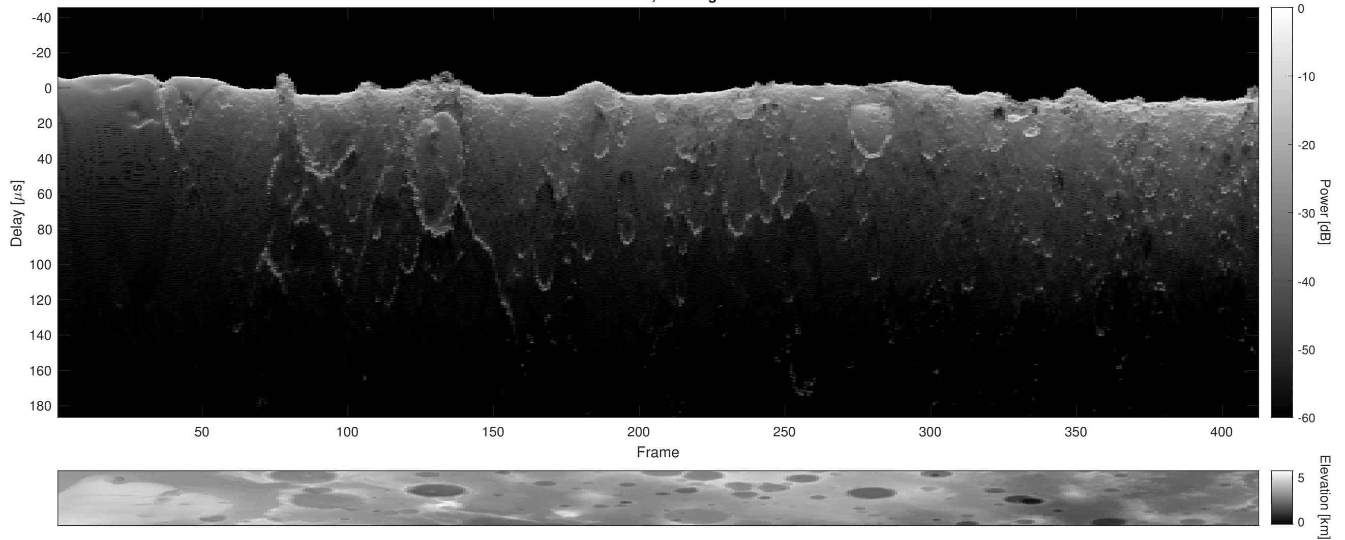
Orbit 15084, Cluttergram
