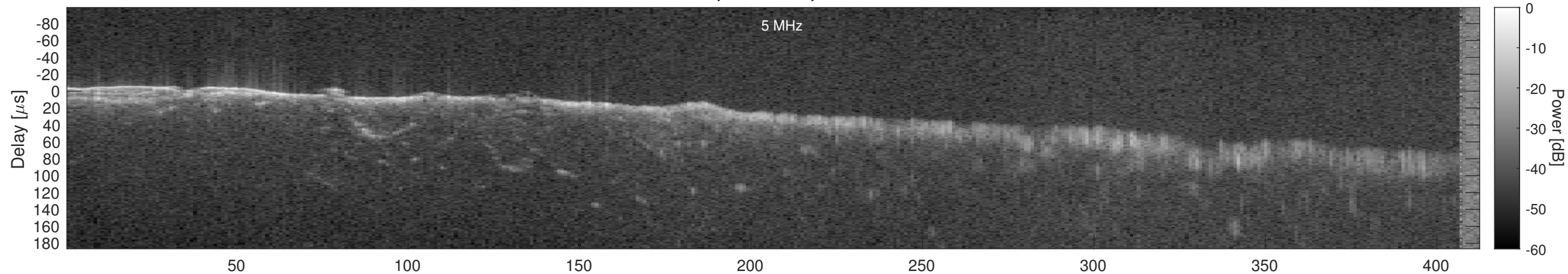
Orbit 15084, Window, Channel 1, Chapman
