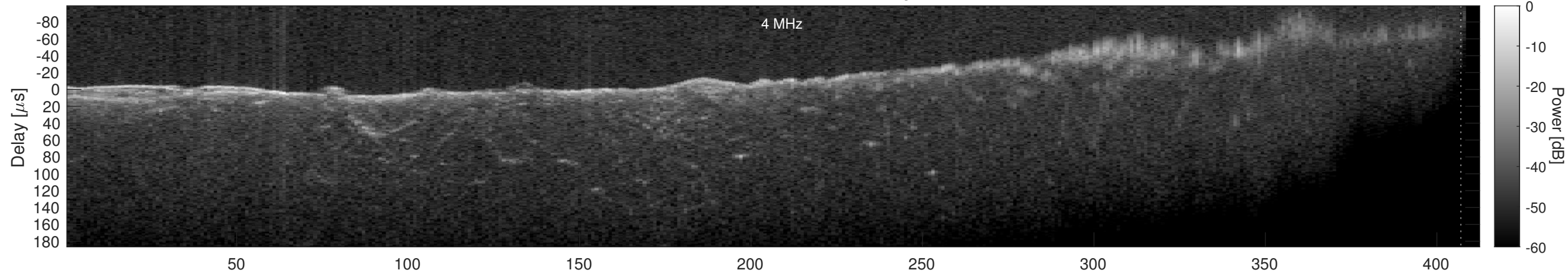
Orbit 15084, Window, Channel 2, Optimized
