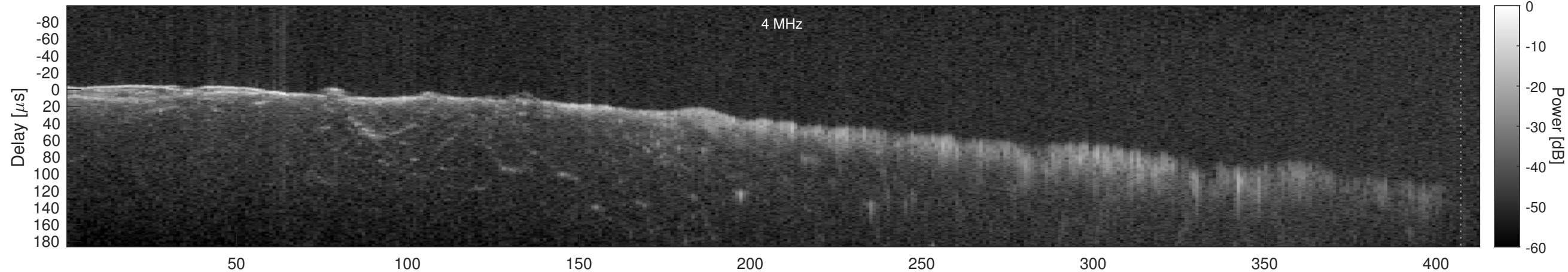
Orbit 15084, Window, Channel 2, Chapman
