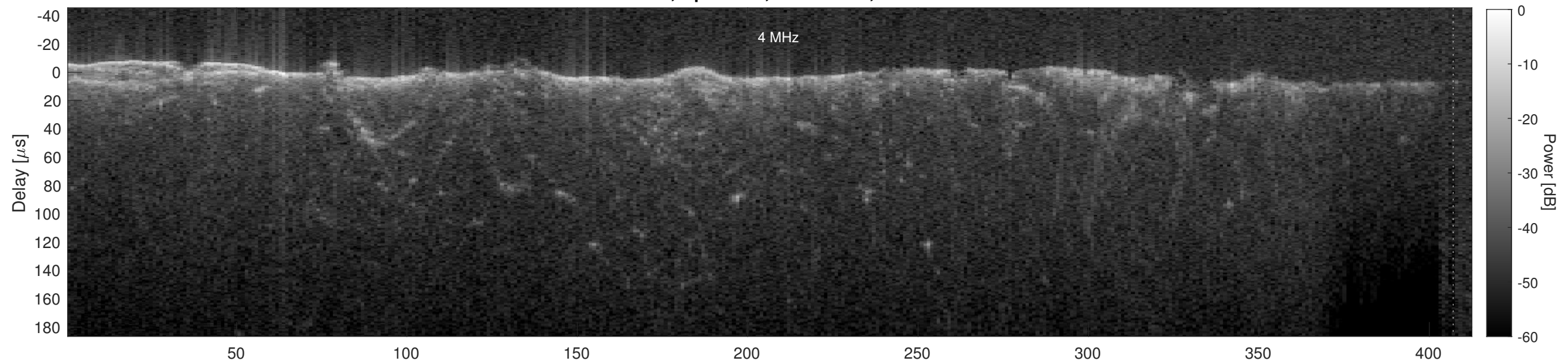
Orbit 15084, Cluttergram
