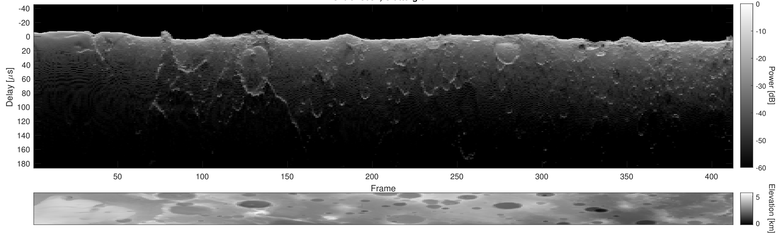
Orbit 15084, Cluttergram
