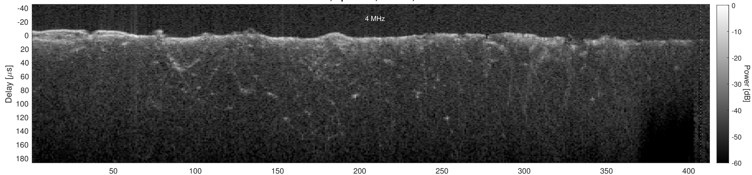
Orbit 15084, Cluttergram
