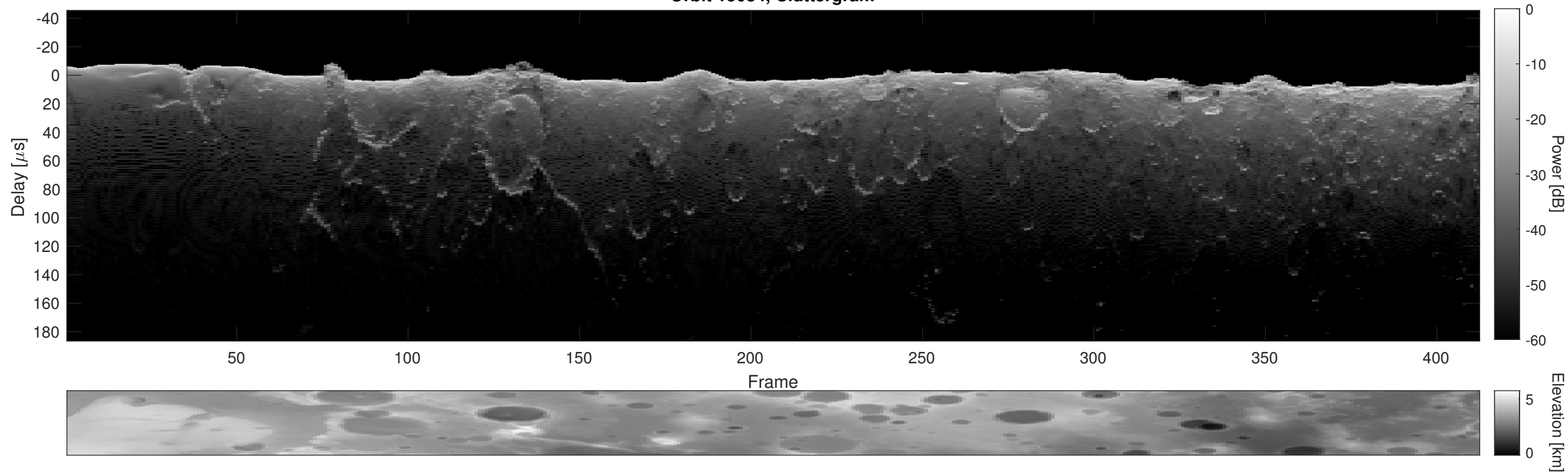
Orbit 15084, Cluttergram
