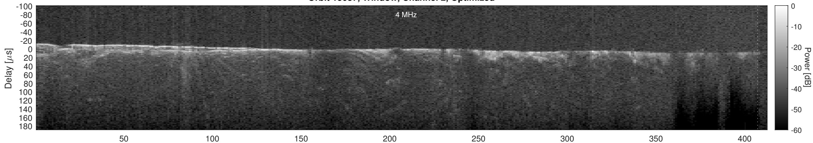
Orbit 15087, Cluttergram
