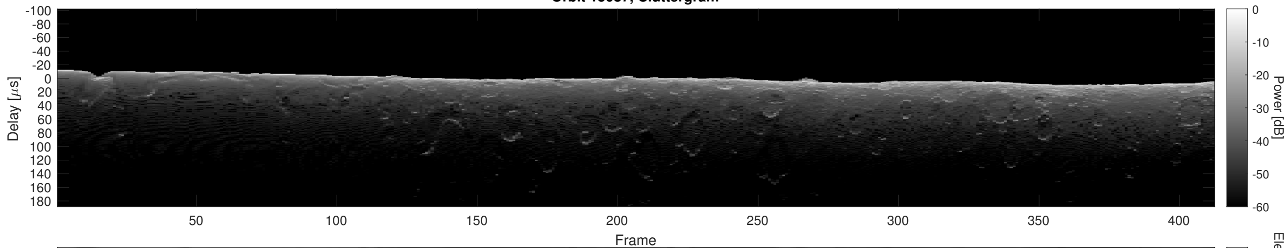
Orbit 15087, Cluttergram
