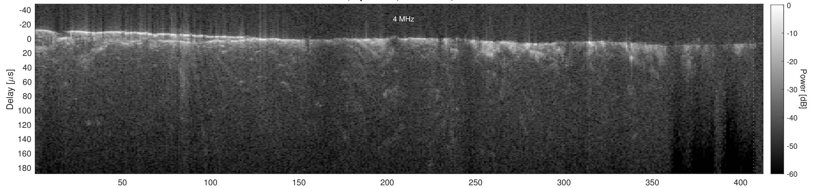
Orbit 15087, Cluttergram
