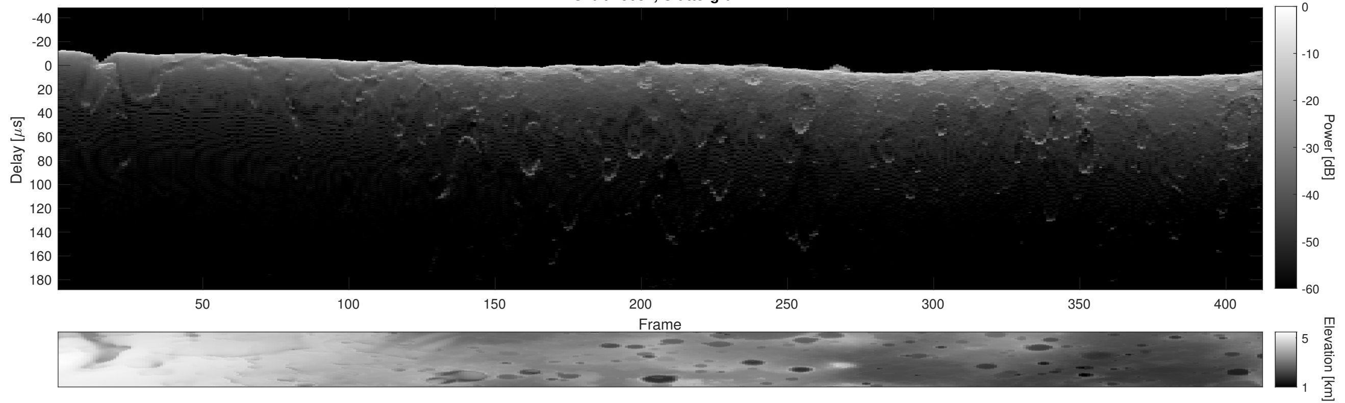
Orbit 15087, Cluttergram
