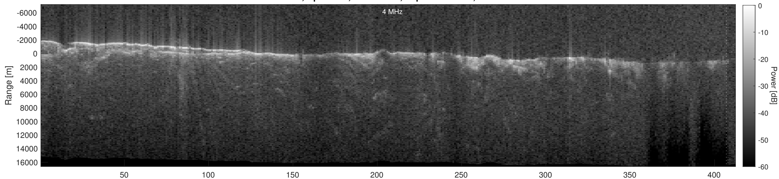
Orbit 15087, Depth-Corrected Cluttergram
