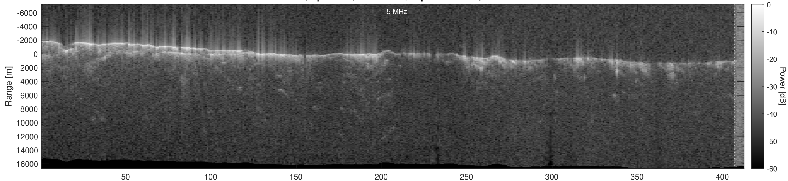
Orbit 15087, Optimized, No Window, Depth-Corrected, Channel 2
