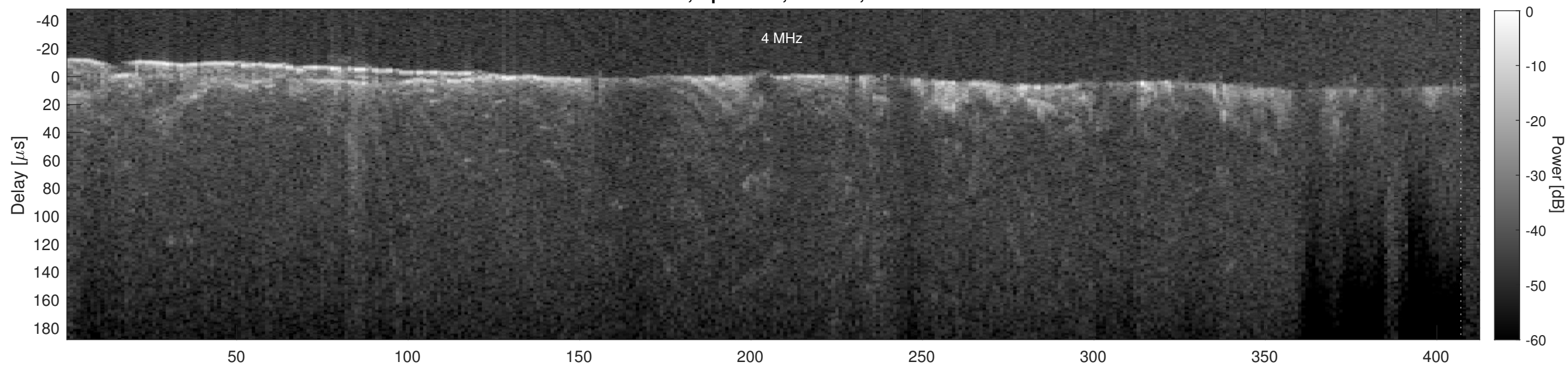
Orbit 15087, Cluttergram
