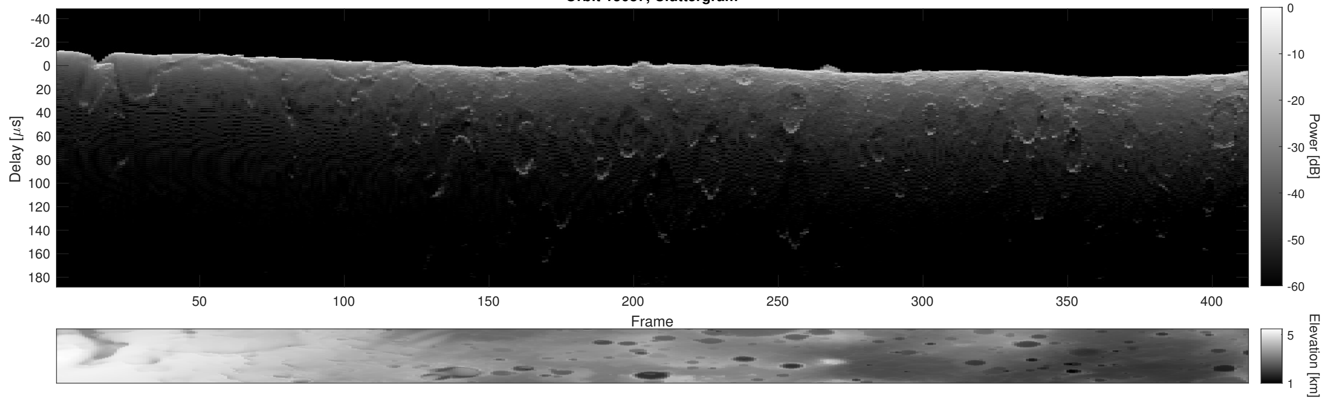
Orbit 15087, Cluttergram
