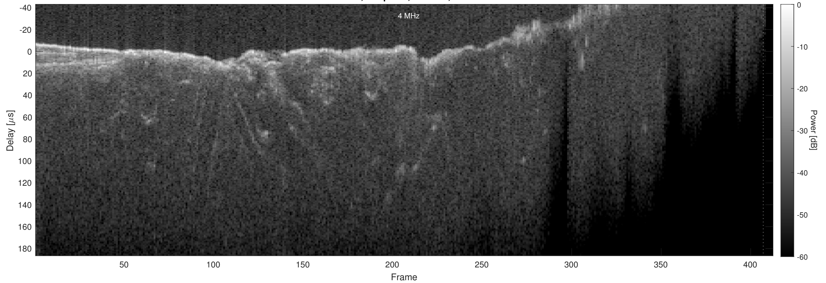
Orbit 15090, Chapman, Window, Channel 2
