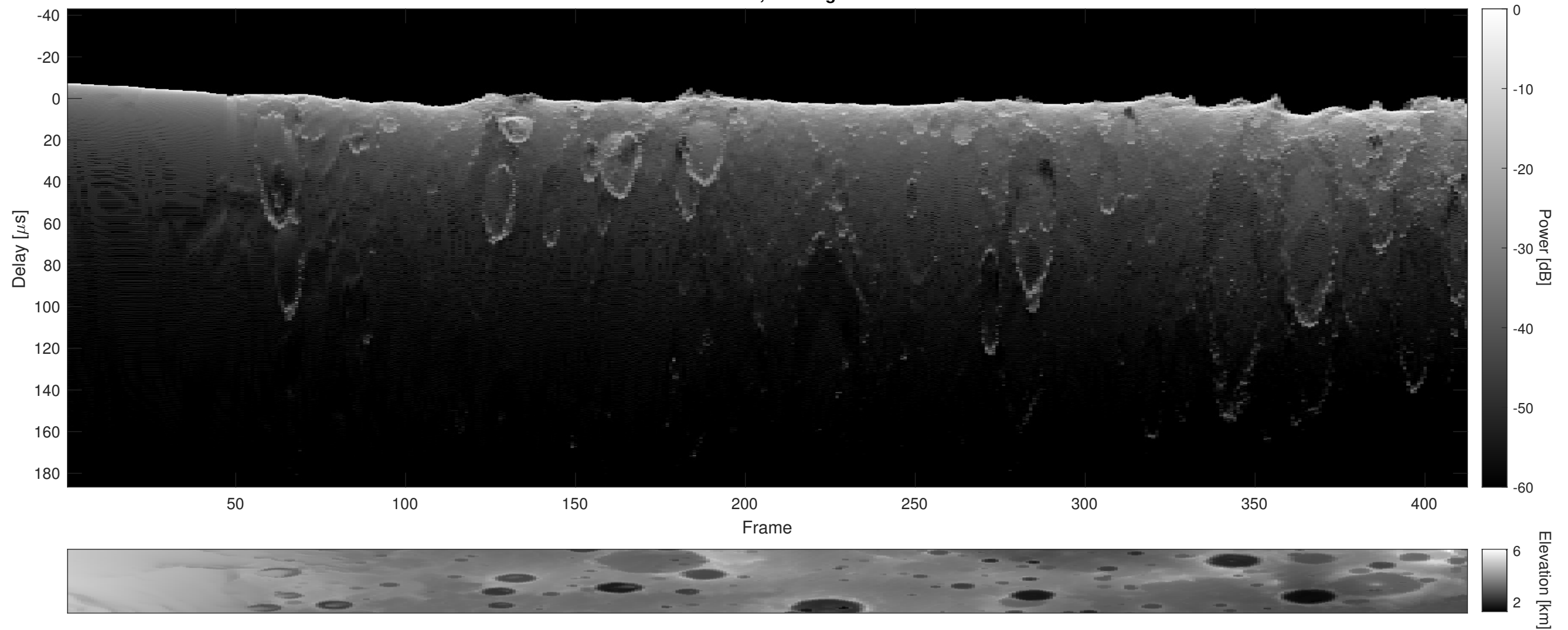
Orbit 15090, Cluttergram
