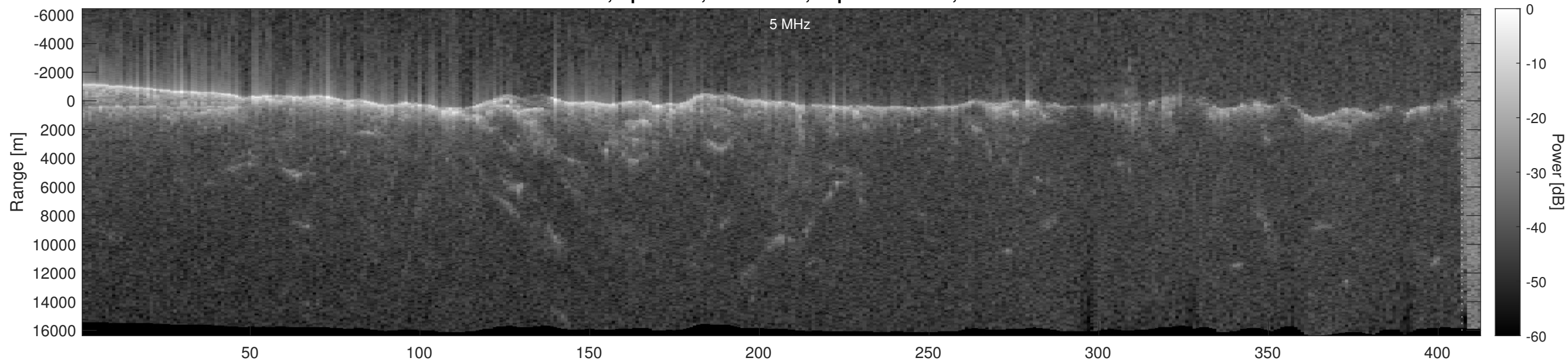
Orbit 15090, Optimized, No Window, Depth-Corrected, Channel 2
