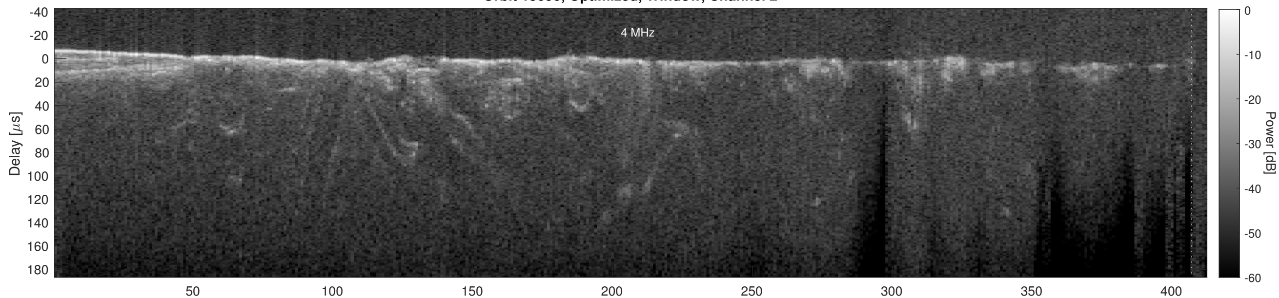
Orbit 15090, Cluttergram
