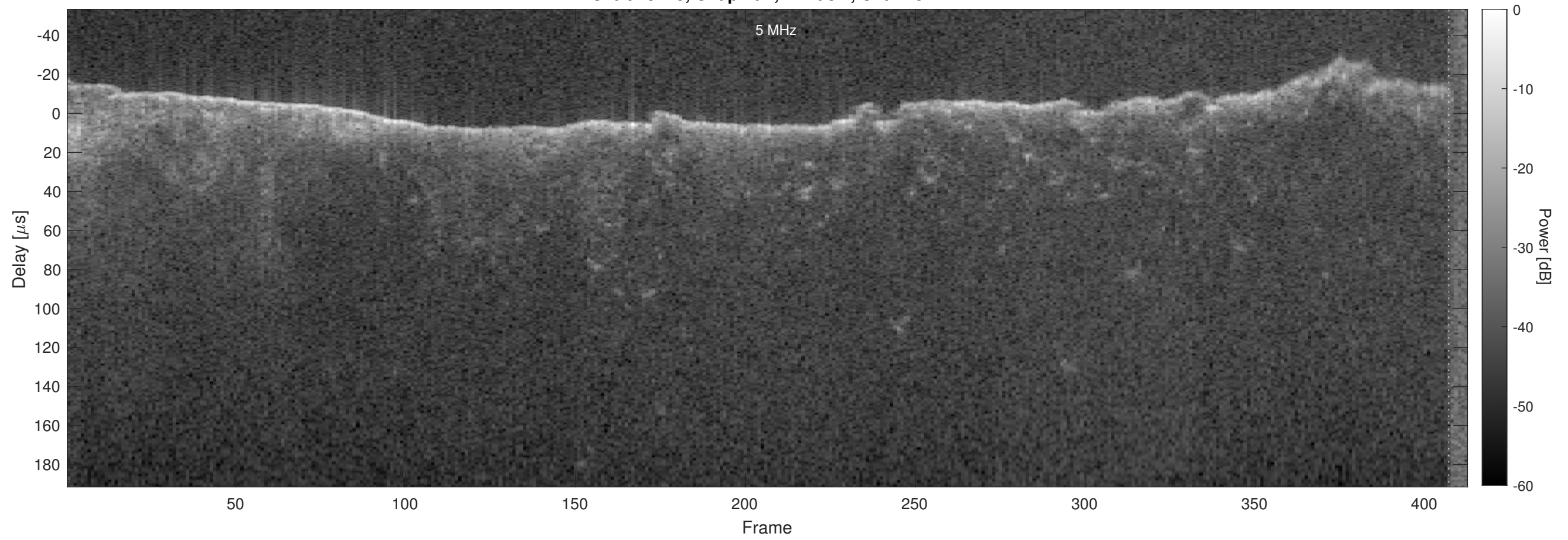
Orbit 15123, Chapman, Window, Channel 2
