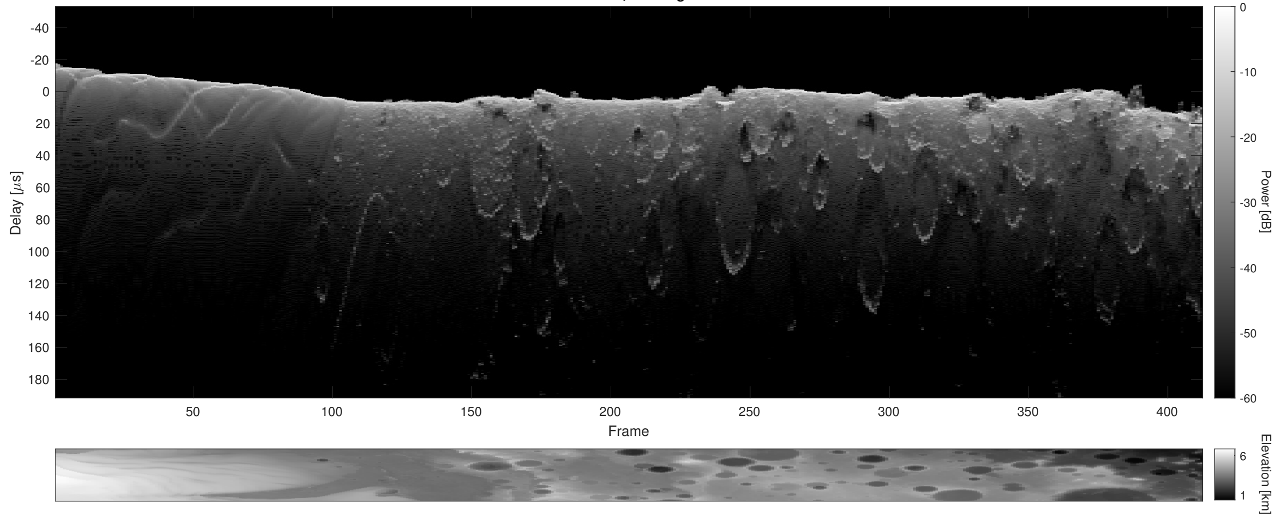
Orbit 15123, Cluttergram
